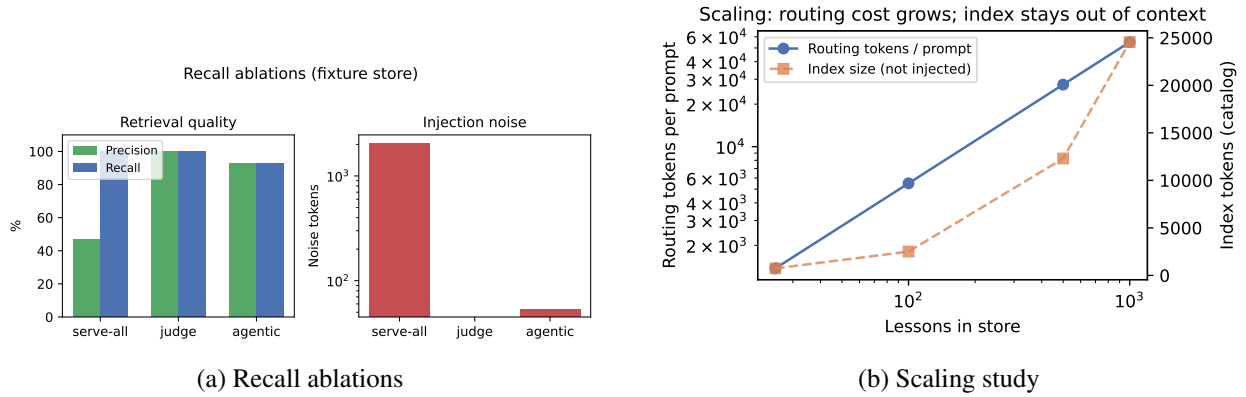
Figure 8: Retrieval filtering removes noise; routing cost scales with store size while index stays out of context.
