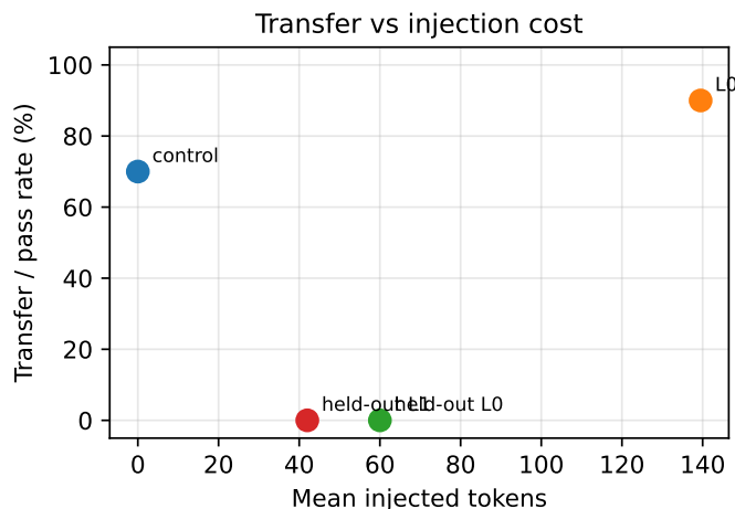
Figure 9: Transfer vs. injection cost on RMC-Bench core cases and held-out retention probe.
