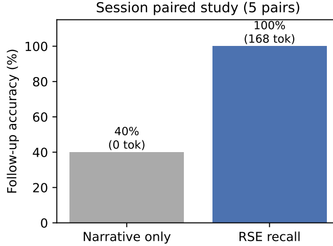
Figure 7: Session paired study: structured recall vs. narrative-only follow-up.
