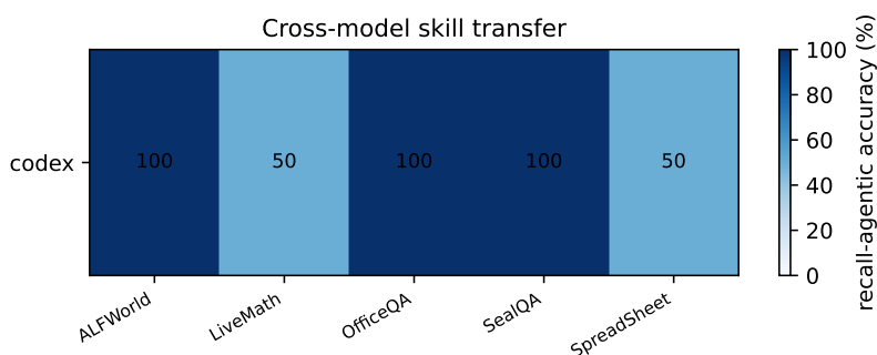
Figure 5: Cross-model transfer: recall-agentic accuracy by inference model (WikiSkill Table 2 style).
