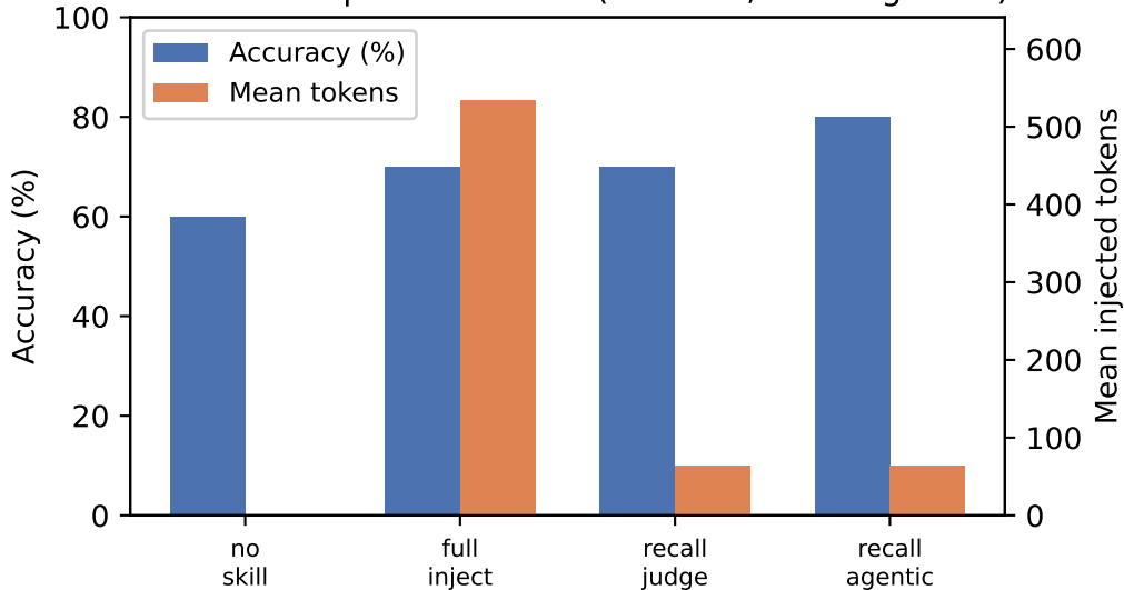
WikiSkill-comparable subset (10 tasks, Codex-graded)
