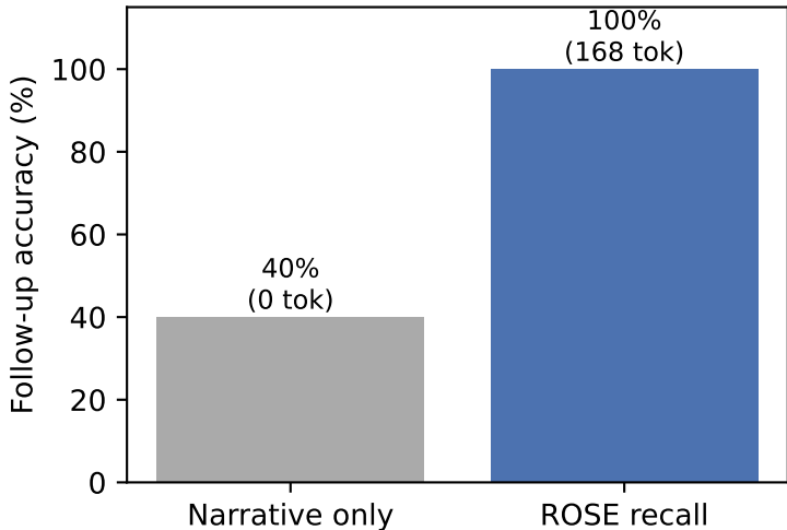
Session paired study (5 pairs)
