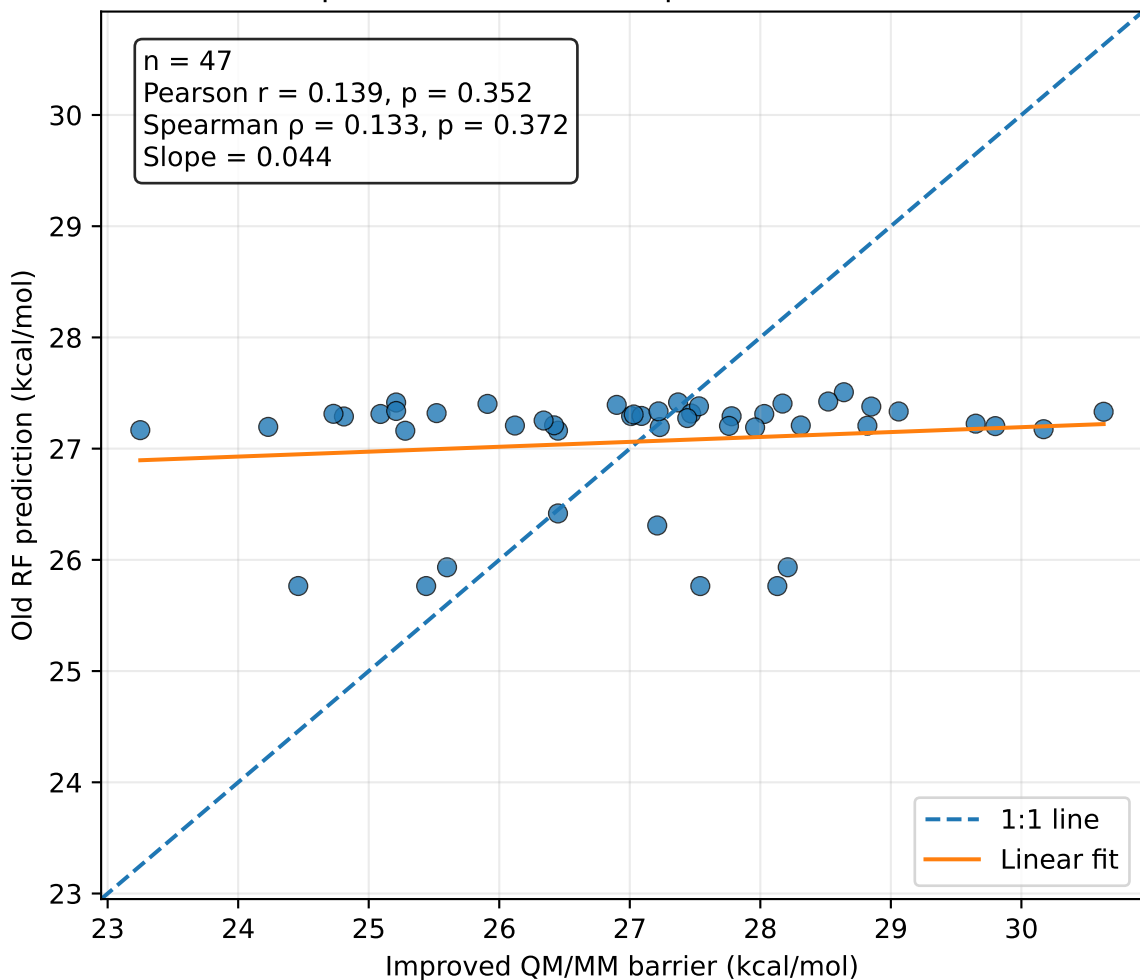
Old RF predictions versus improved QM/MM barriers
