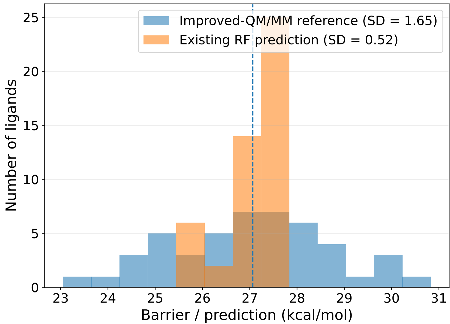
Distributions of improved-QM/MM barriers and existing RF predictions
