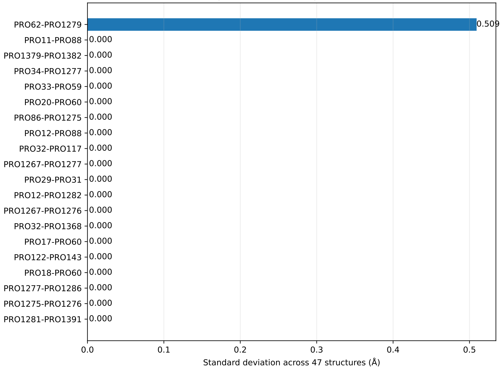
Variability of the 20 most important RF features
