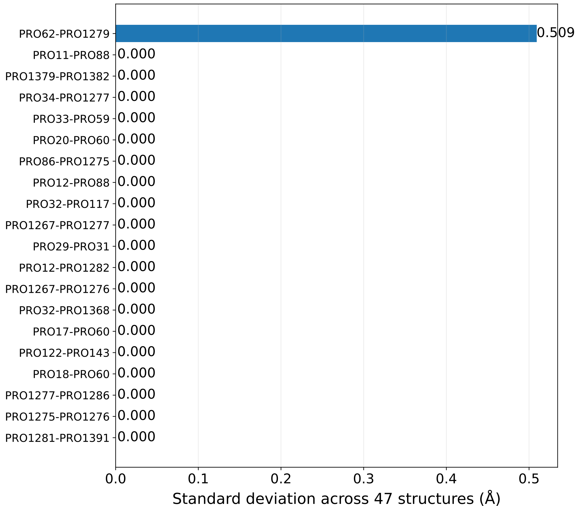
Variability of the 20 most important existing RF features
