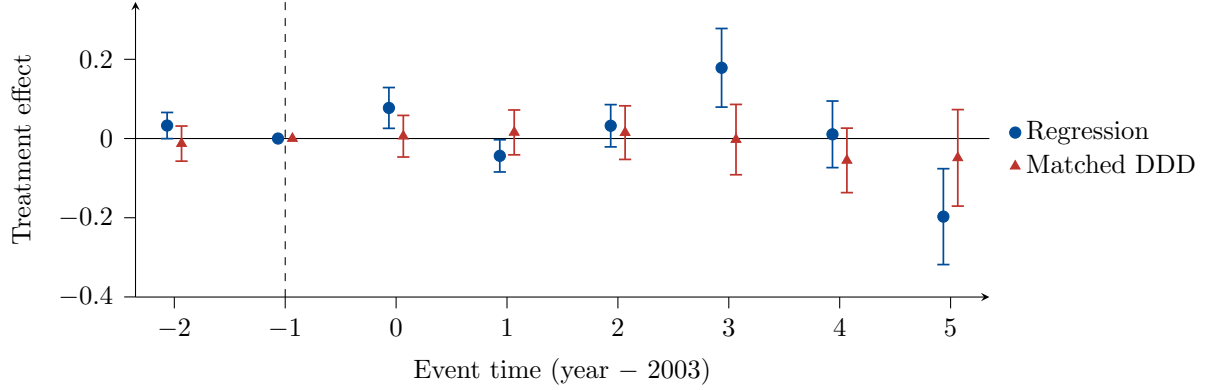
Figure 10: Matched DDD and Regression event studies: Bias-corrected Nearest-neighbor matching.
