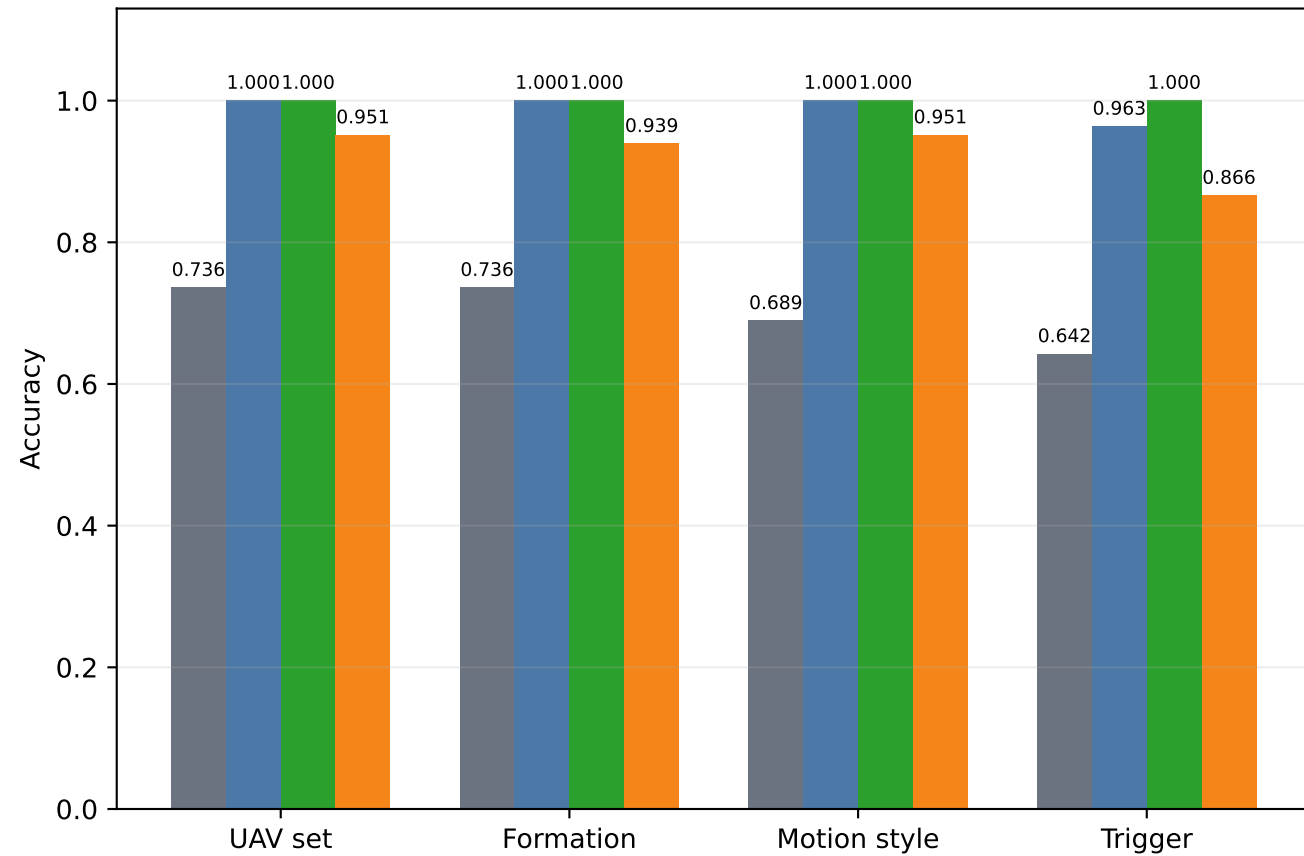
Semantic Field Accuracy
