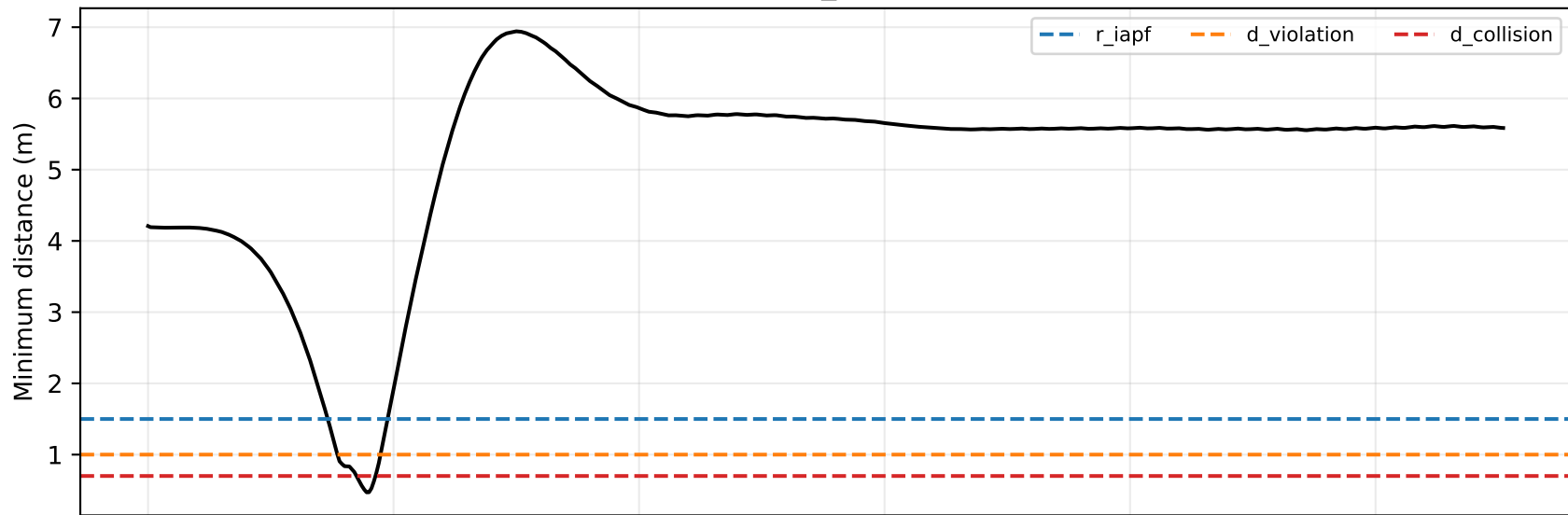
IAPF_OFF
