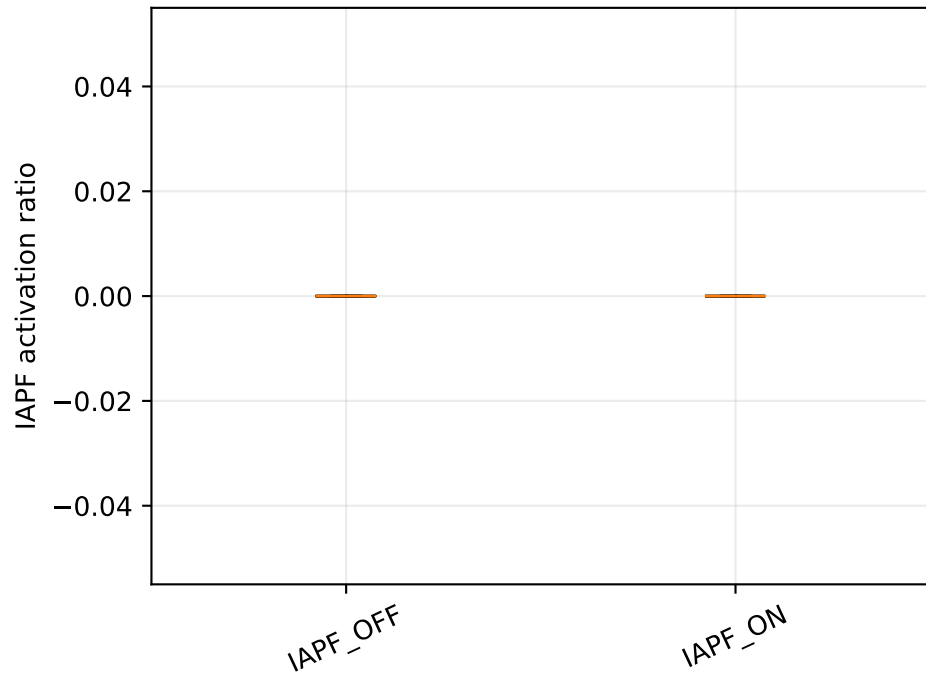
safe_wide_line_to_circle
