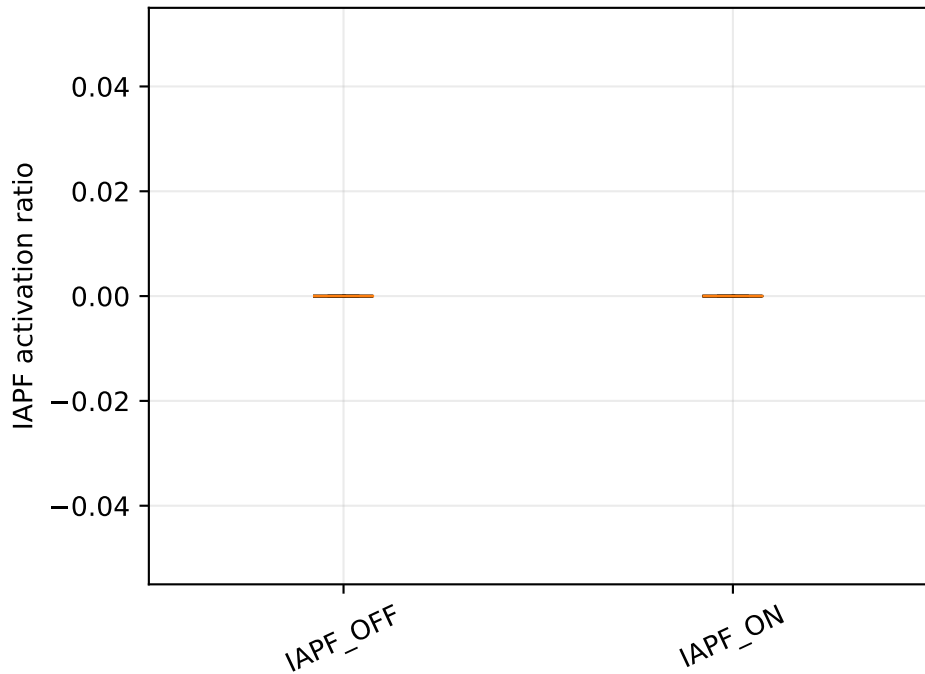
safe_parallel_groups
