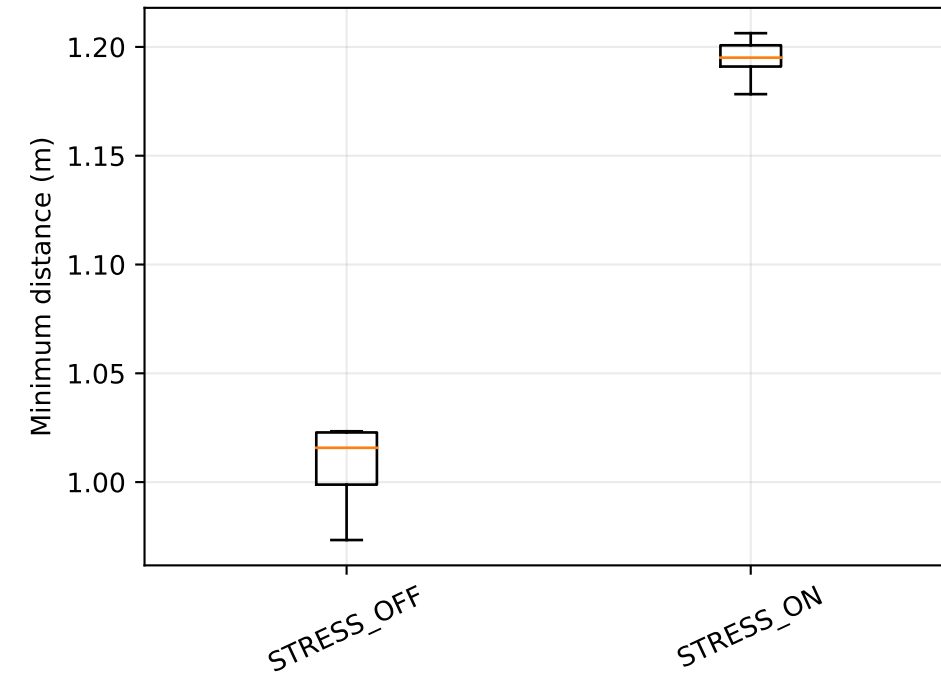
dense_infeasible
