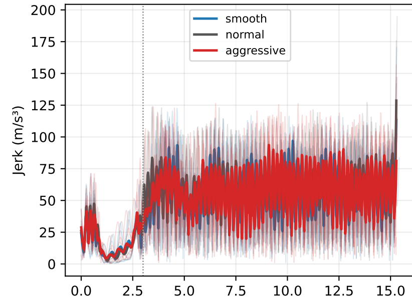
Jerk (m/s 3 )
