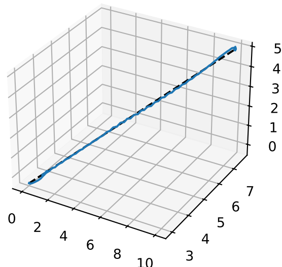
eight_uav_line_to_circle linear_ladrc
