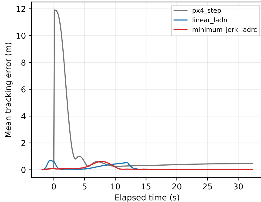
eight uav line to circle
