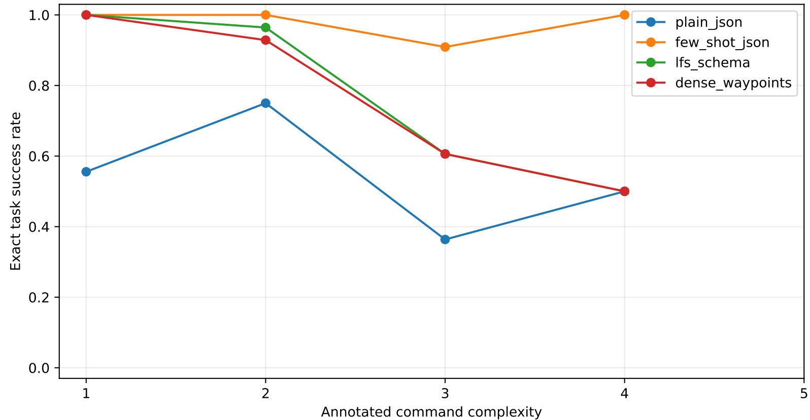
Command Complexity vs Parsing Success
