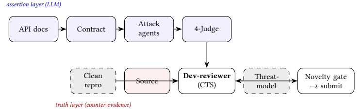
Figure 1: TestVDB pipeline. The assertion layer (LLM contract + 4-judge) is falsified by the dev-reviewer’s three counter-evidence anchors (truth layer): the source anchor is validated in our retrospective, while the reproduction and threat-model anchors (gray, dashed) are design-level and not yet evaluated. CTS = Contract-Truth Separation.
