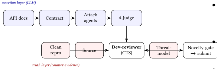
Figure 1: TestVDB pipeline. The assertion layer (LLM contract + 4-judge) is falsified by the dev-reviewer’s three counter-evidence anchors (truth layer). CTS = Contract-Truth Separation.
