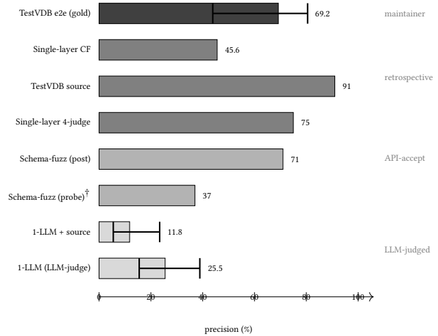
Figure 2: Precision by ground-truth tier (darker = stronger). Whiskers = Wilson 95% CI; † = probe \rightarrow accept rate, not candidate precision. Details in Table 5.
