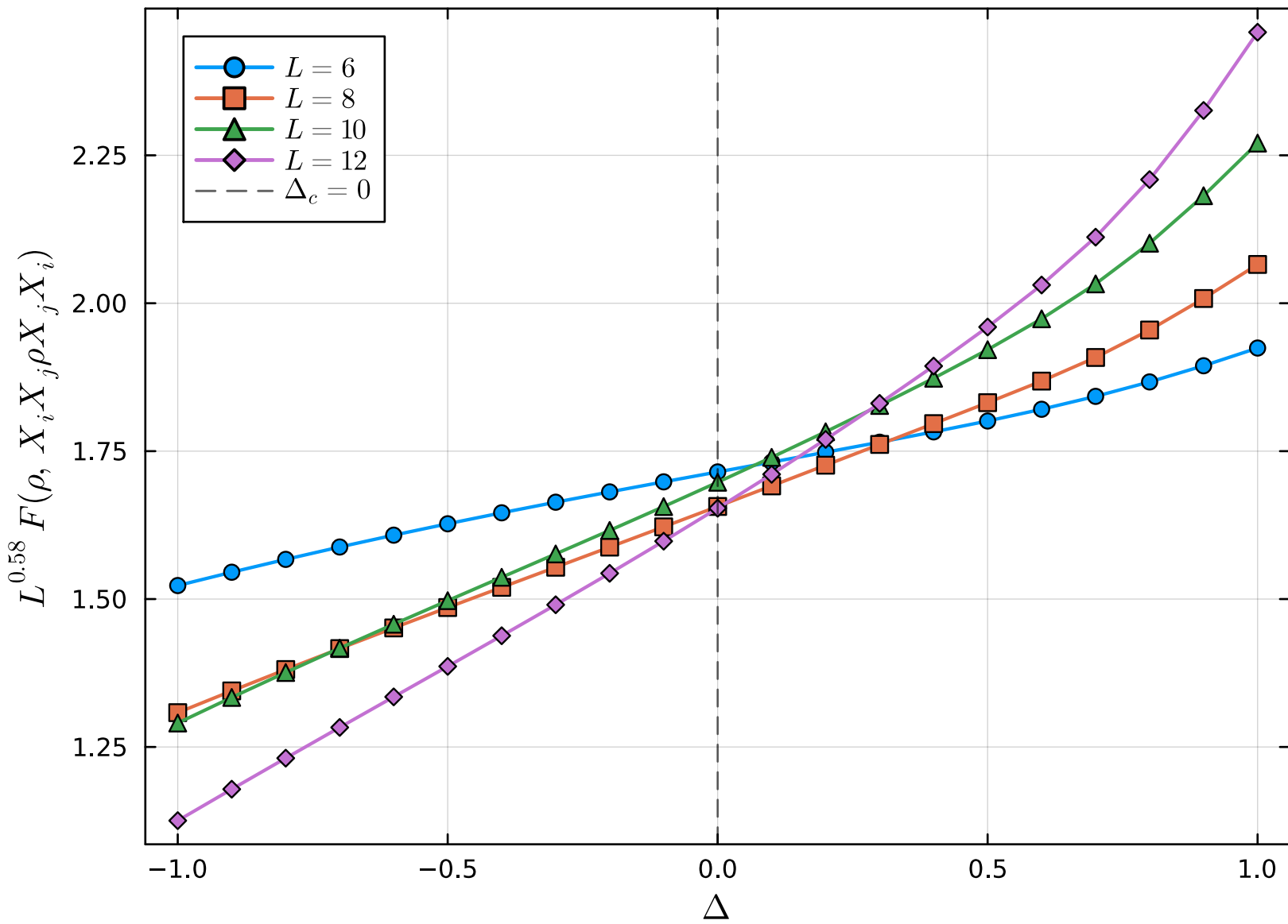
Uhlmann fidelity, p = 0.05 , PBC -- rescaled
