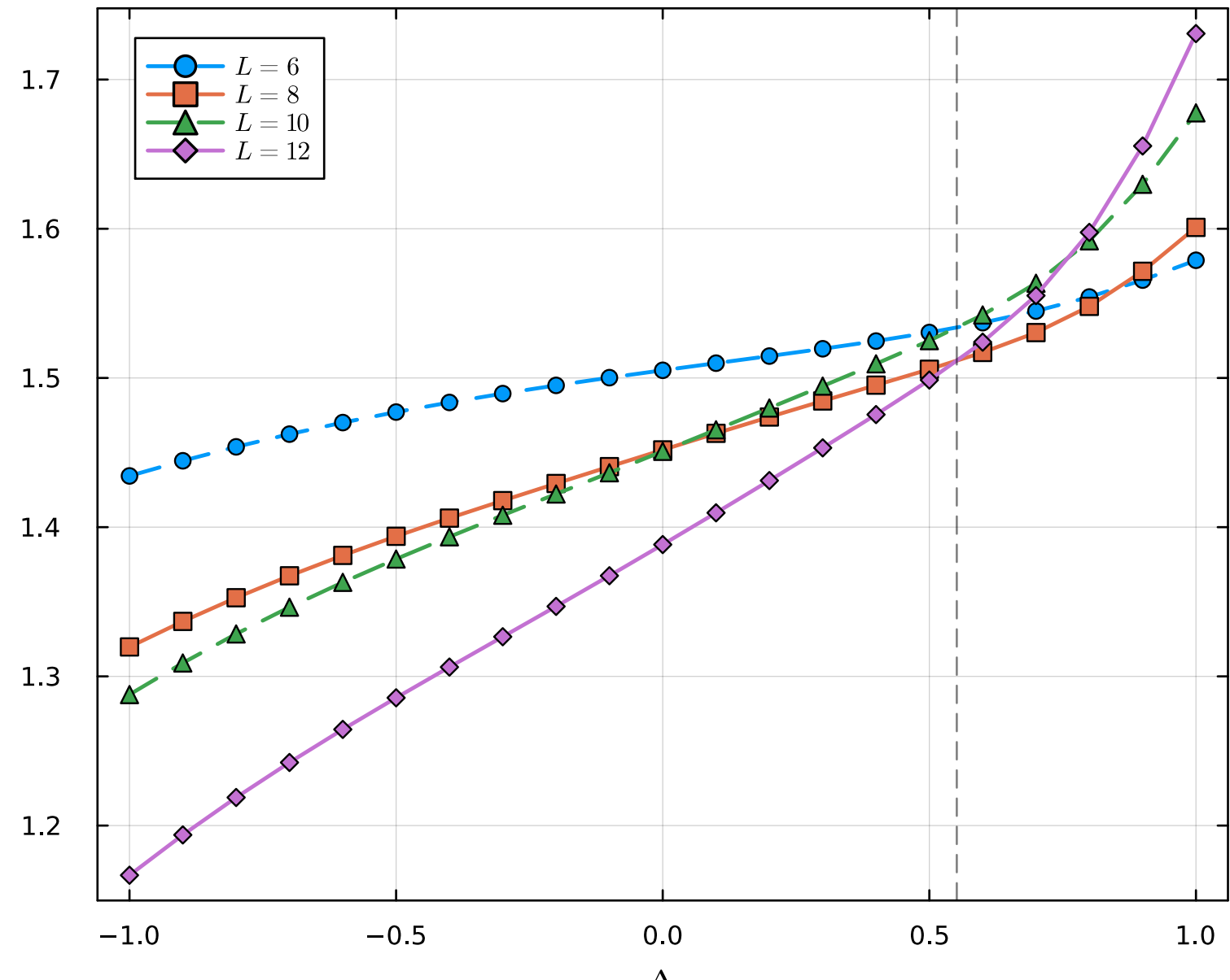
rescaled with the crossing exponent
