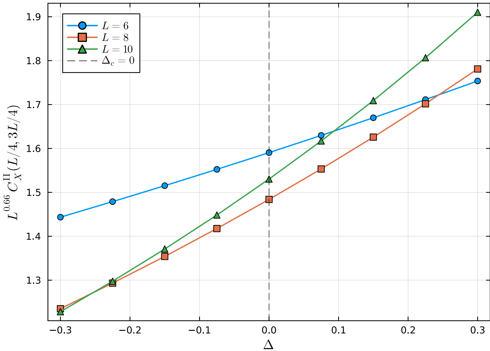
XXZ under XX decoherence, p = 0.1 , PBC
