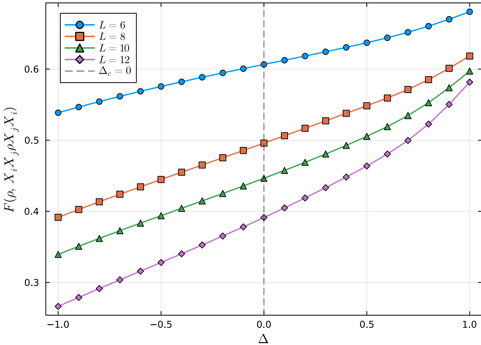
Uhlmann fidelity, p = 0.05 , PBC -- raw
