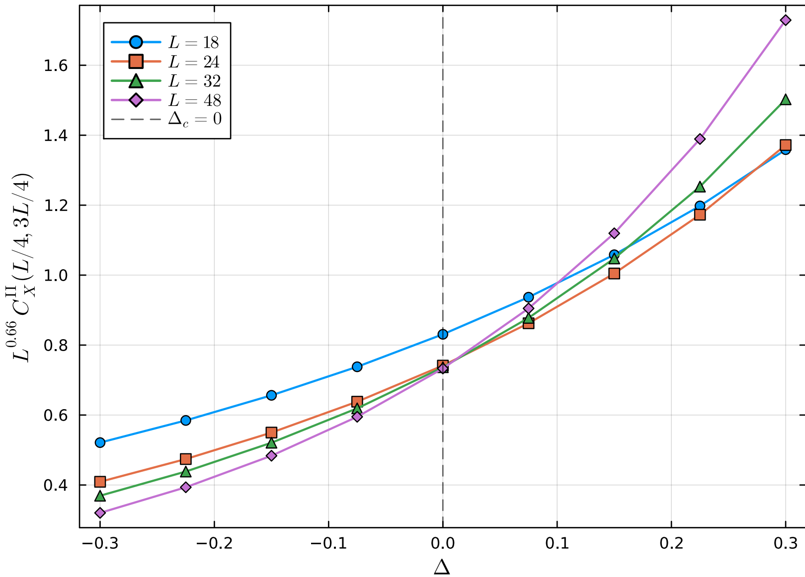
XXZ under XX decoherence, p = 0.1 , OBC
