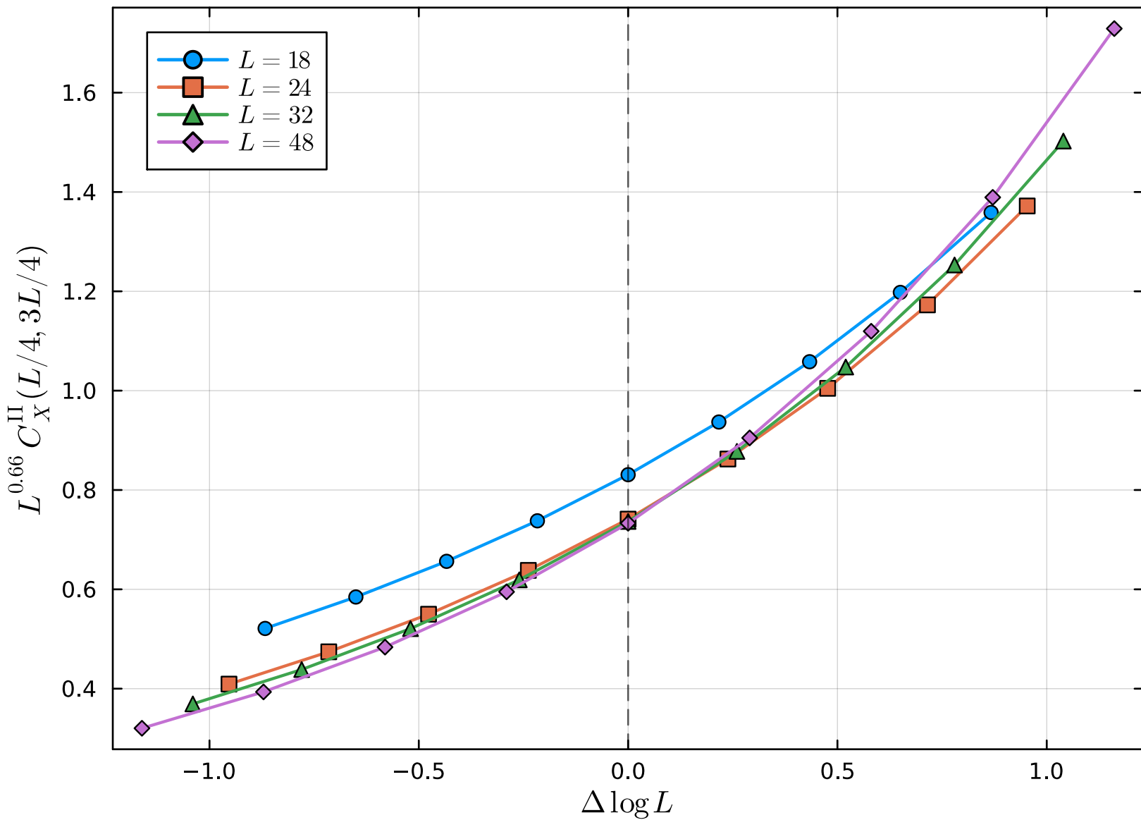
data collapse (boundary BKT), p = 0.1 , OBC
