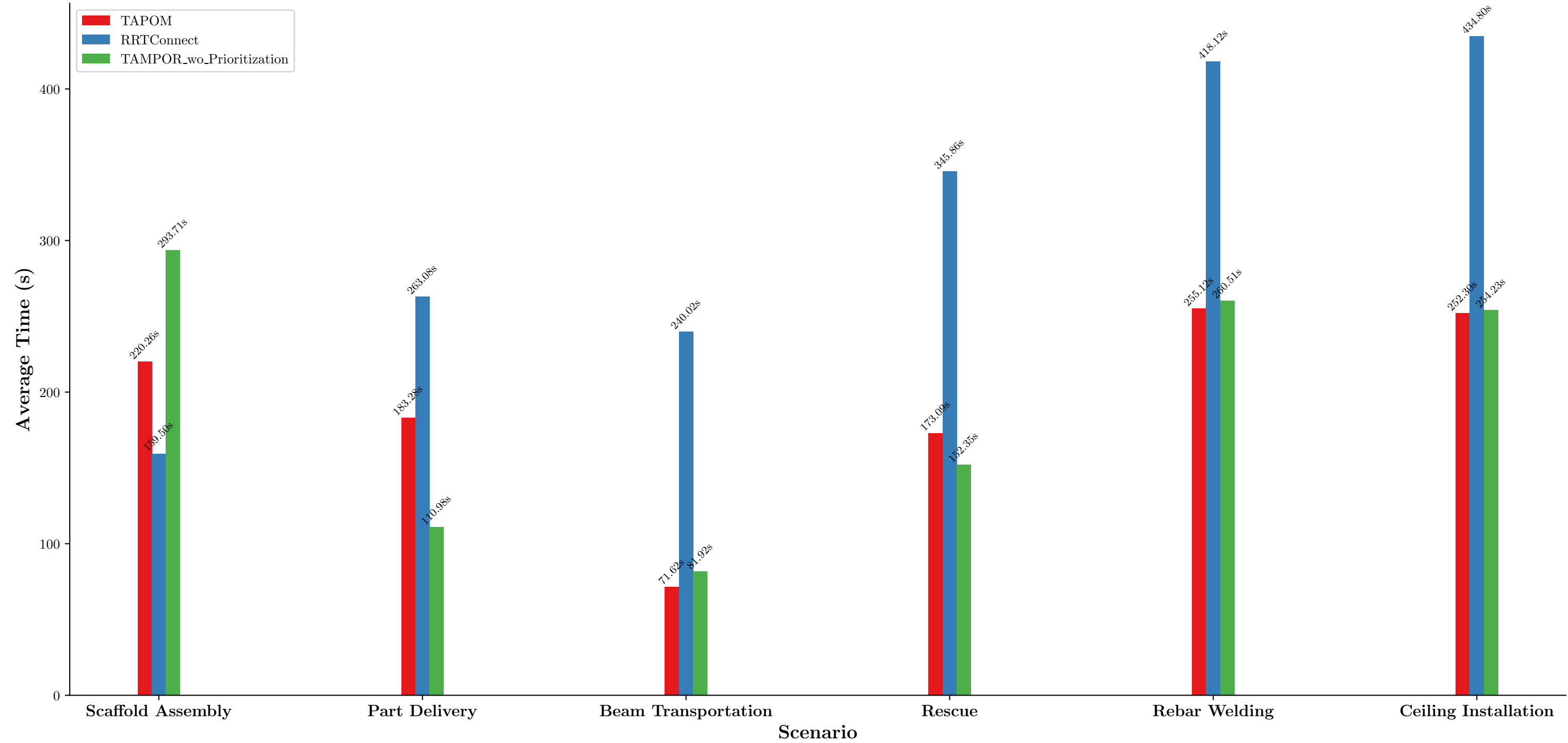
Average Planning Time for Successful Trials Only
