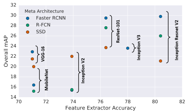
Fig. 13: A comparison of detection accuracy of three detectors: Faster RCNN [19], R-FCN [49] and SSD [23] on MS-COCO dataset with different detection backbones. Image from J. Huang et al. CVPR 2017 [186].
