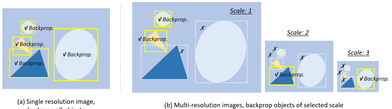
Fig. 12: Different training strategies for multi-scale object detection: (a): Training on a single resolution image, back propagate objects of all scales [17–19, 23]. (b) Training on multi-resolution images (image pyramid), back propagate objects of selected scale. If an object is too large or too small, its gradient will be discarded [39, 176, 177].
