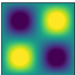
Fr-PINN-elm [1, 2] (20, 20)
