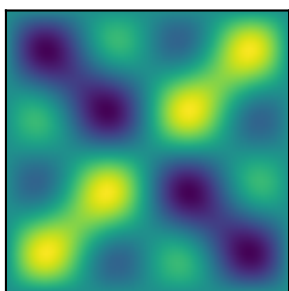
Fr-PINN-elm [1, 2, 4] (40, 40)
