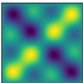
FBPINN [1, 2, 4] (40, 40)
