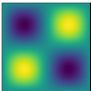
Exact solution
