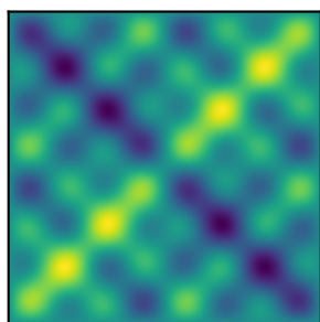
FBPINN [1, 2, 4, 8] (80, 80)
