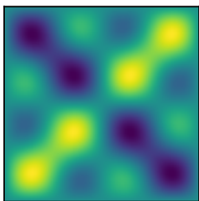
Exact solution
