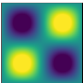
Fr-PINN-swim [1, 2] (20, 20)
