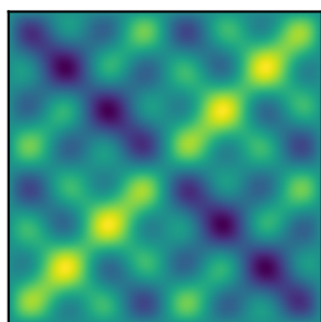
Fr-PINN-elm [1, 2, 4, 8] (80, 80)
