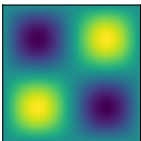
FBPINN [1, 2] (20, 20)
