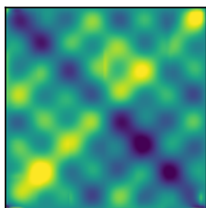
Fr-PINN-swim [1, 2, 4, 8] (80, 80)
