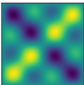
Fr-PINN-swim [1, 2, 4] (40, 40)
