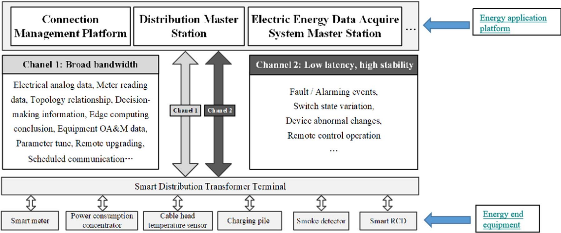
Figure A.4.8-1: Example of a smart distribution transformer terminal workflow
