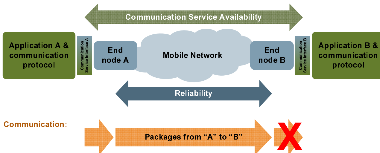
Figure F-2: Example in which reliability and communication service availability have different values. Packages are reliably transmitted from the communication service interface A to end node B, but they are not exposed at the communication service interface B.
