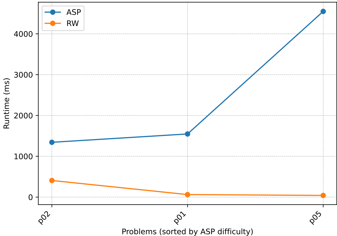
logistics - runtime_ms
