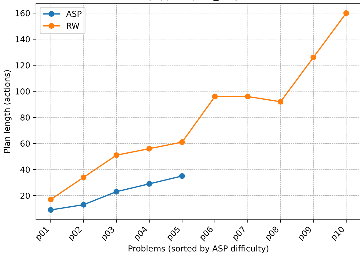
gripper - plan_length
