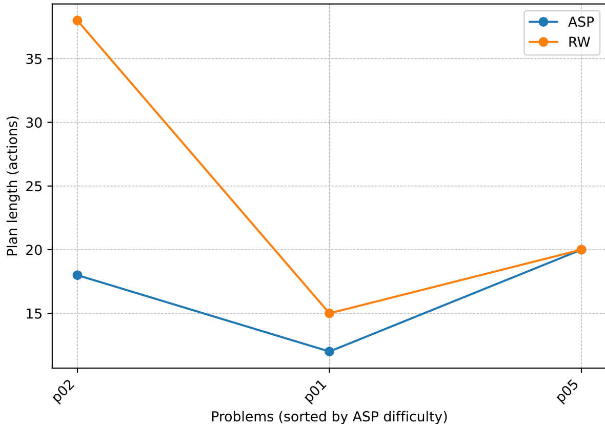
logistics - plan_length
