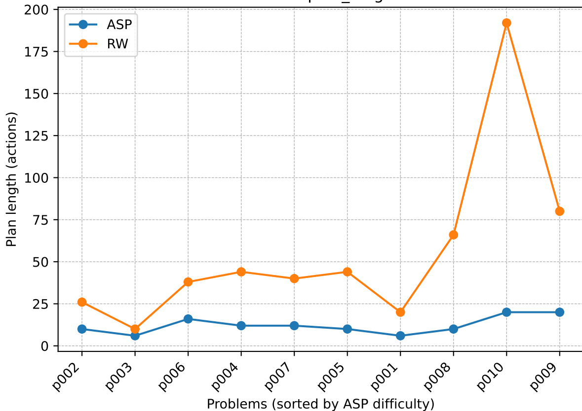
blocks - plan_length
