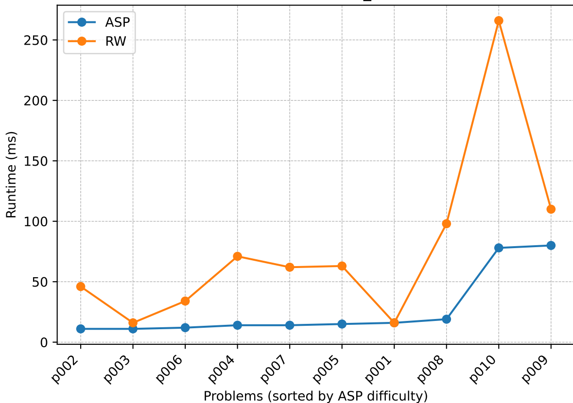
blocks - runtime_ms
