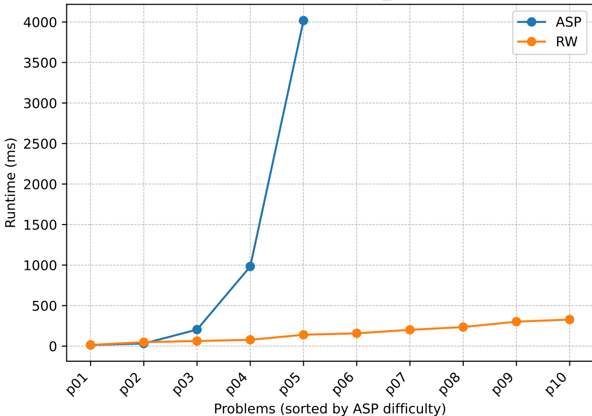
gripper - runtime_ms
