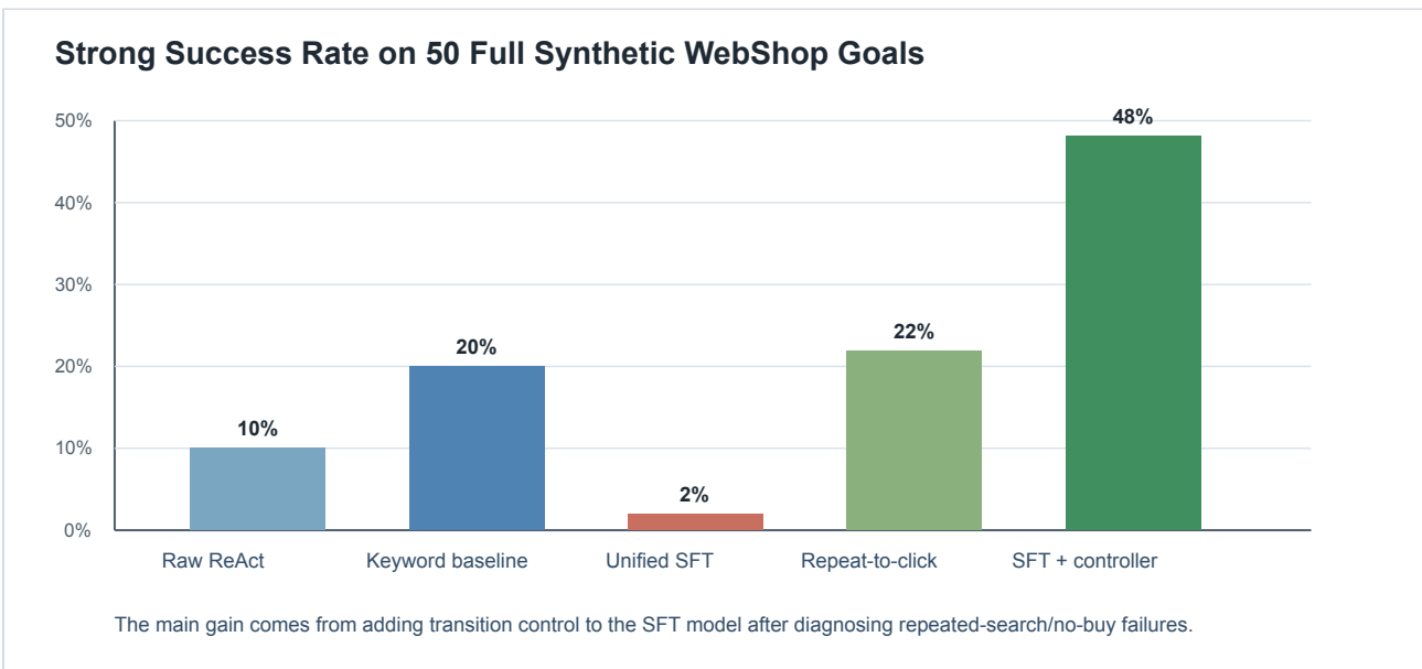
Figure 2: Strong success rate on 50 full synthetic WebShop goals. SFT alone underperforms, while controller-guided SFT gives the best result.
