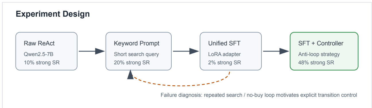
Figure 1: Experimental workflow from raw ReAct to keyword prompting, SFT, failure diagnosis, and controller-guided SFT.
