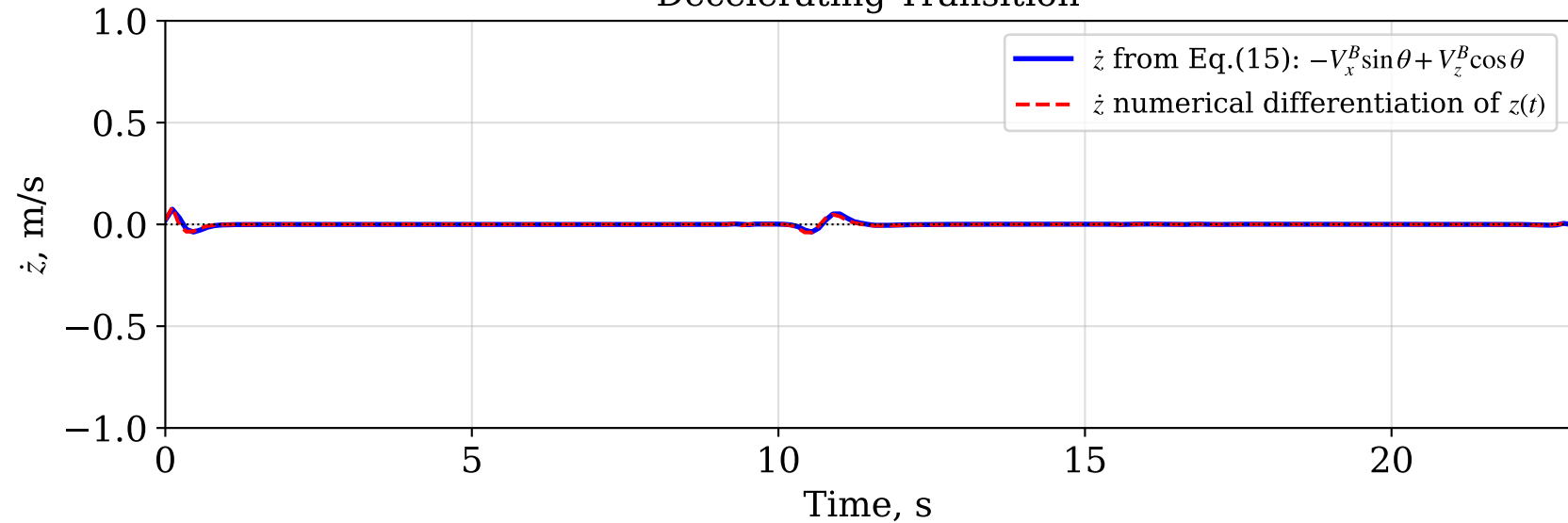
Decelerating Transition
