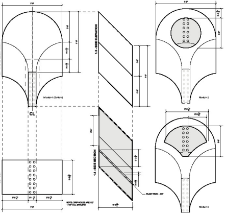
Fabrication Drawings
