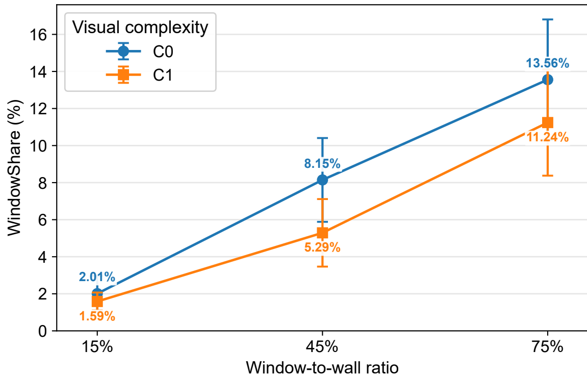
B. WindowShare by WWR and visual complexity
