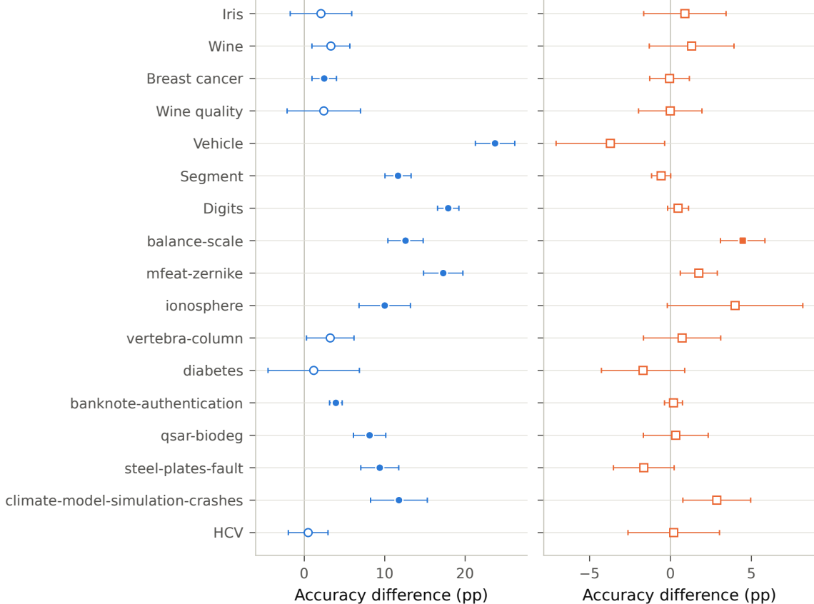
(a) Trained – untrained encoder
