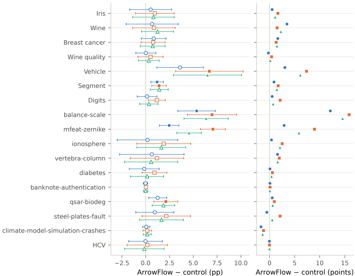
(a) Accuracy difference (pp)
