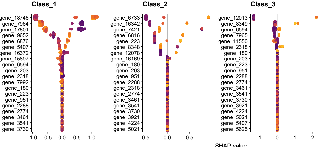
TreeSHAP — XGBoost
