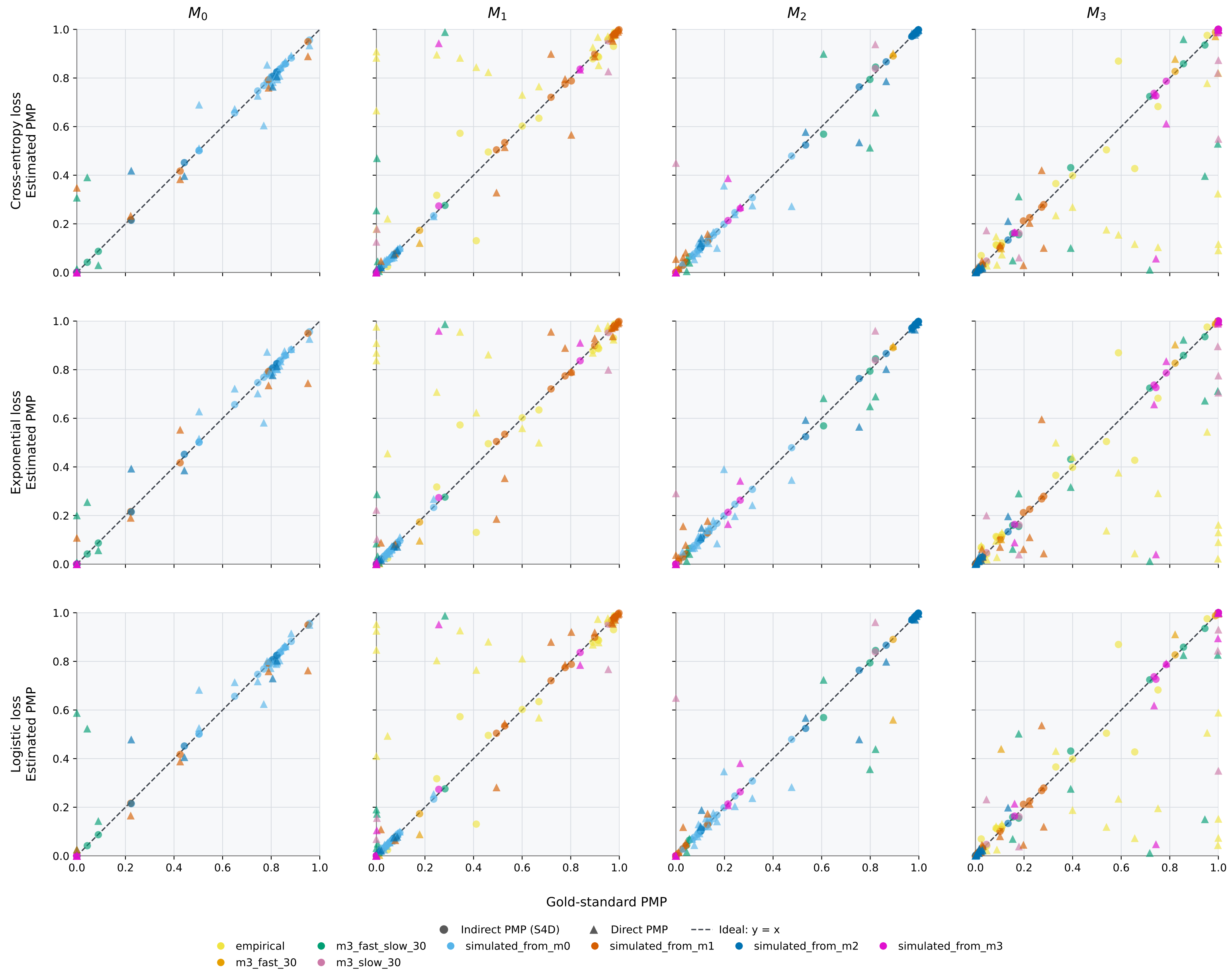
Posterior model probability recovery by data source
