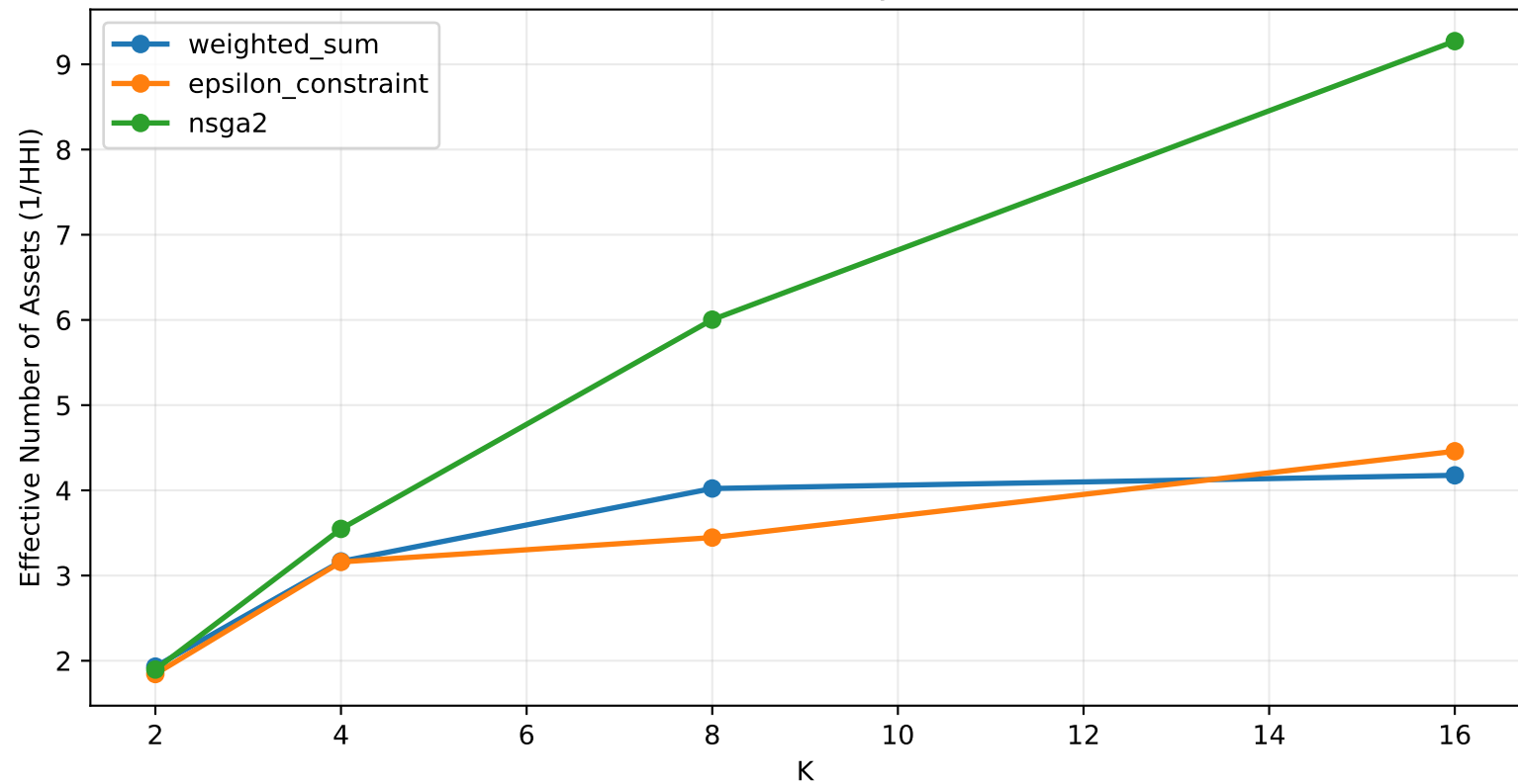
Diversification vs Cardinality (Balanced Point)
