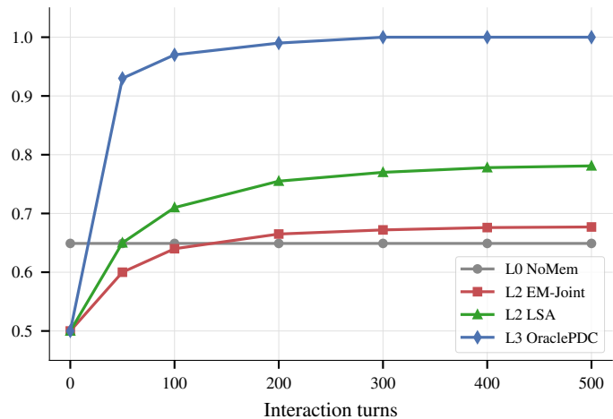
GPT-5.4 (strong, 82% MMLU)
