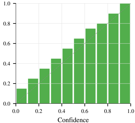
Claude-Opus-4-6 (conservative, ECE=0.158)
