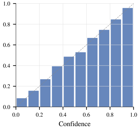
Qwen-Turbo (calibrated, ECE=0.165)
