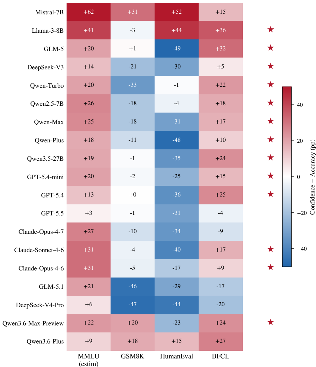
Cross-task Gap sign matrix (★ = sign flip in protocol-controlled subset, 13/19)
