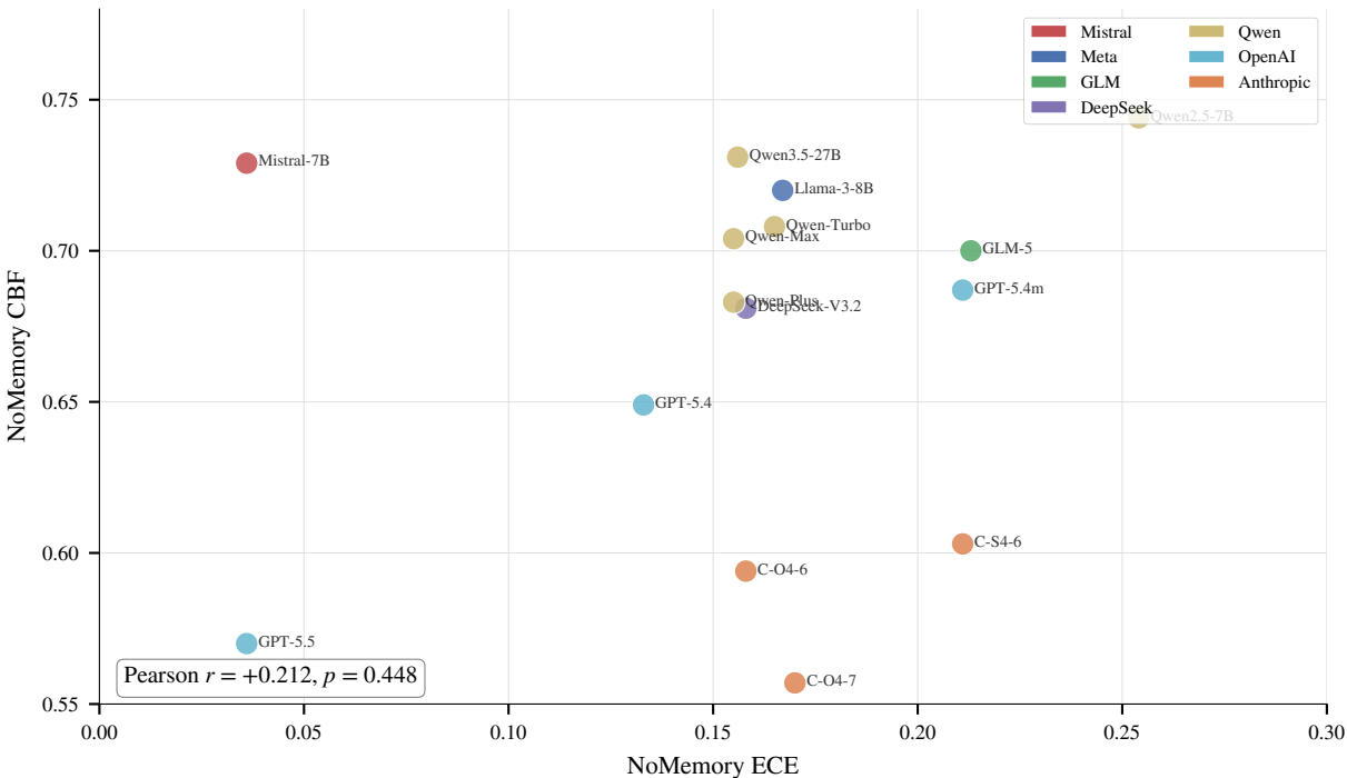
CBF and ECE measure different aspects of self-knowledge
