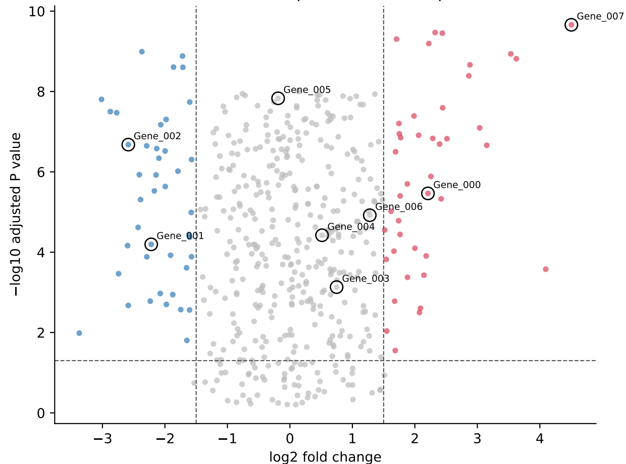
Differential expression volcano plot
