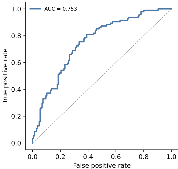
Model A
