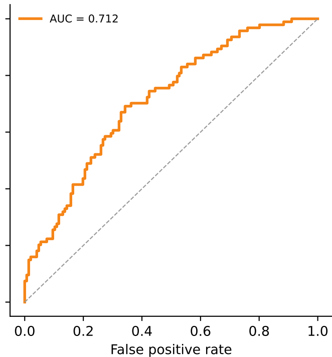
Model B
