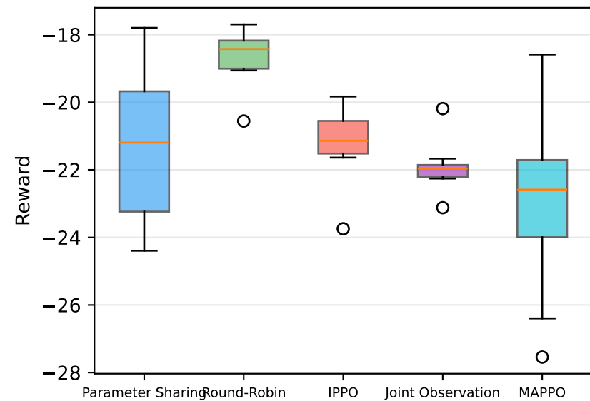
Reward spread (last 25% of evals)
