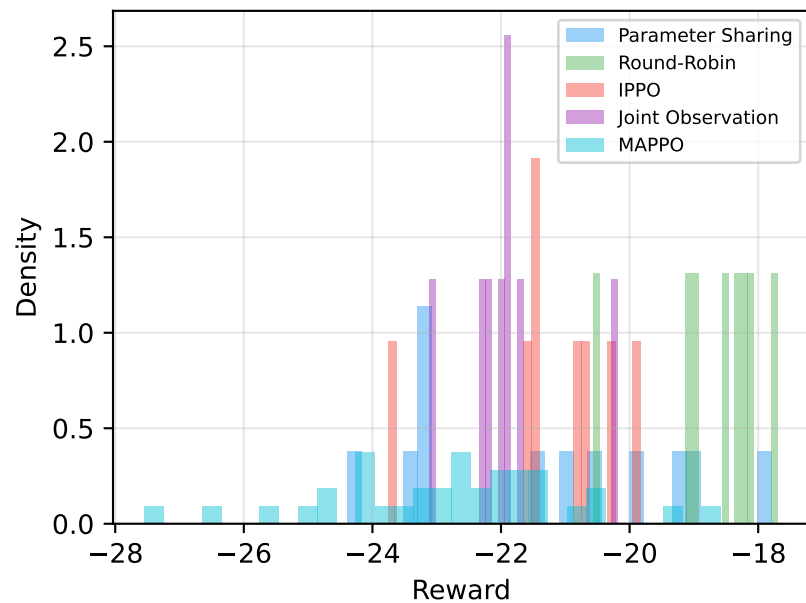
Reward distribution (last 25% of evals)
