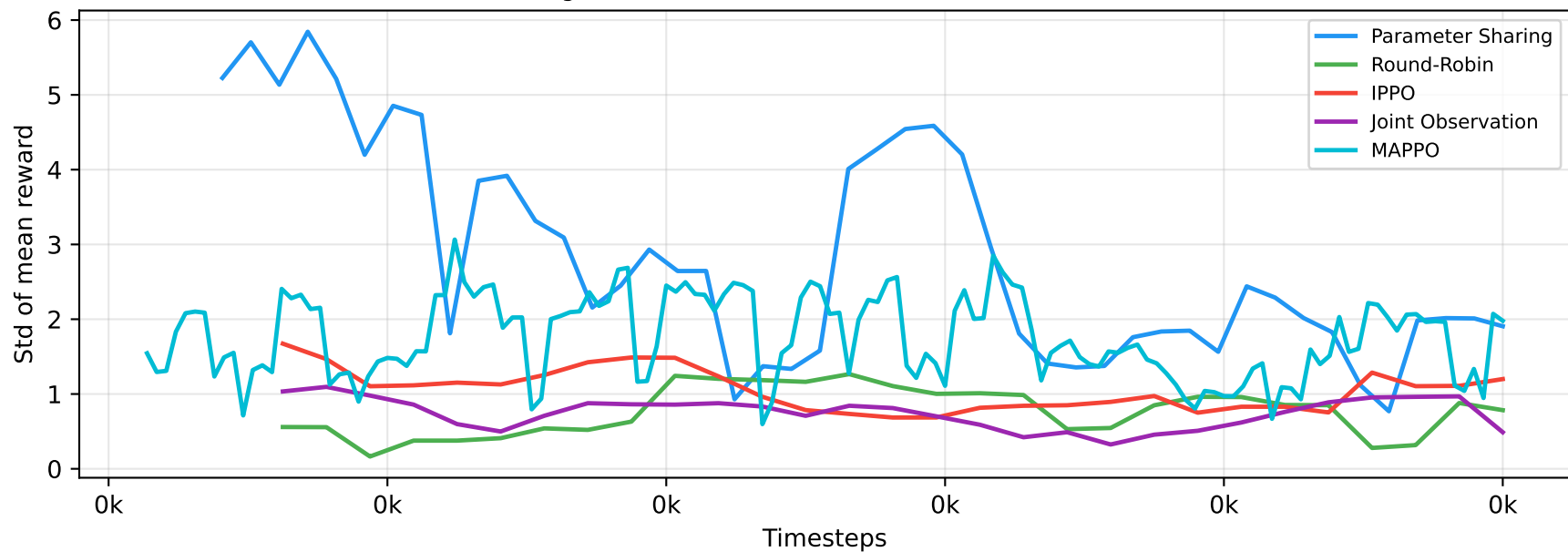
Rolling reward std (window=5) — lower = more stable
