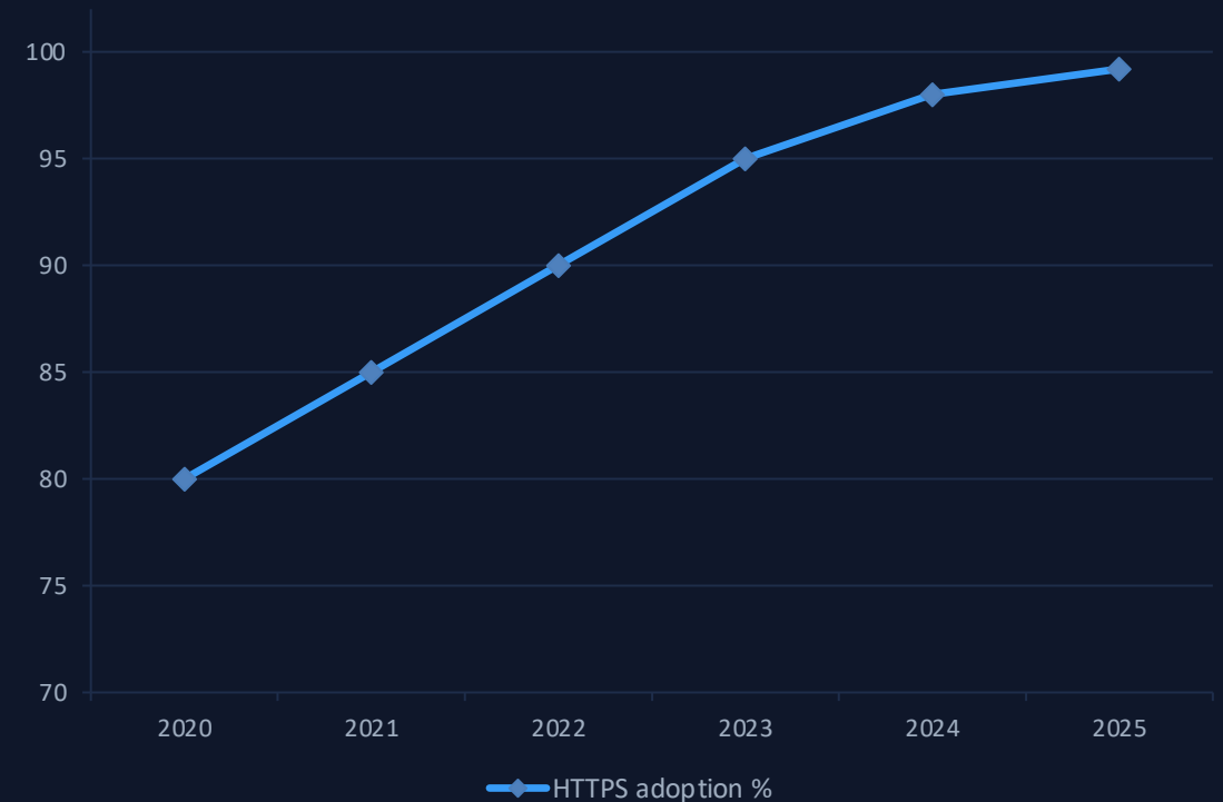
HTTPS adoption %
