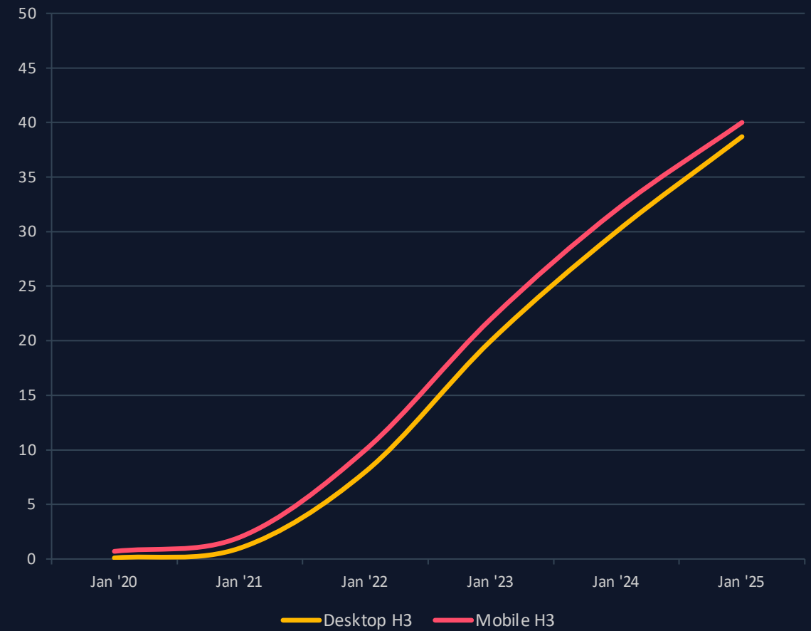
HTTP/3 support time-series
