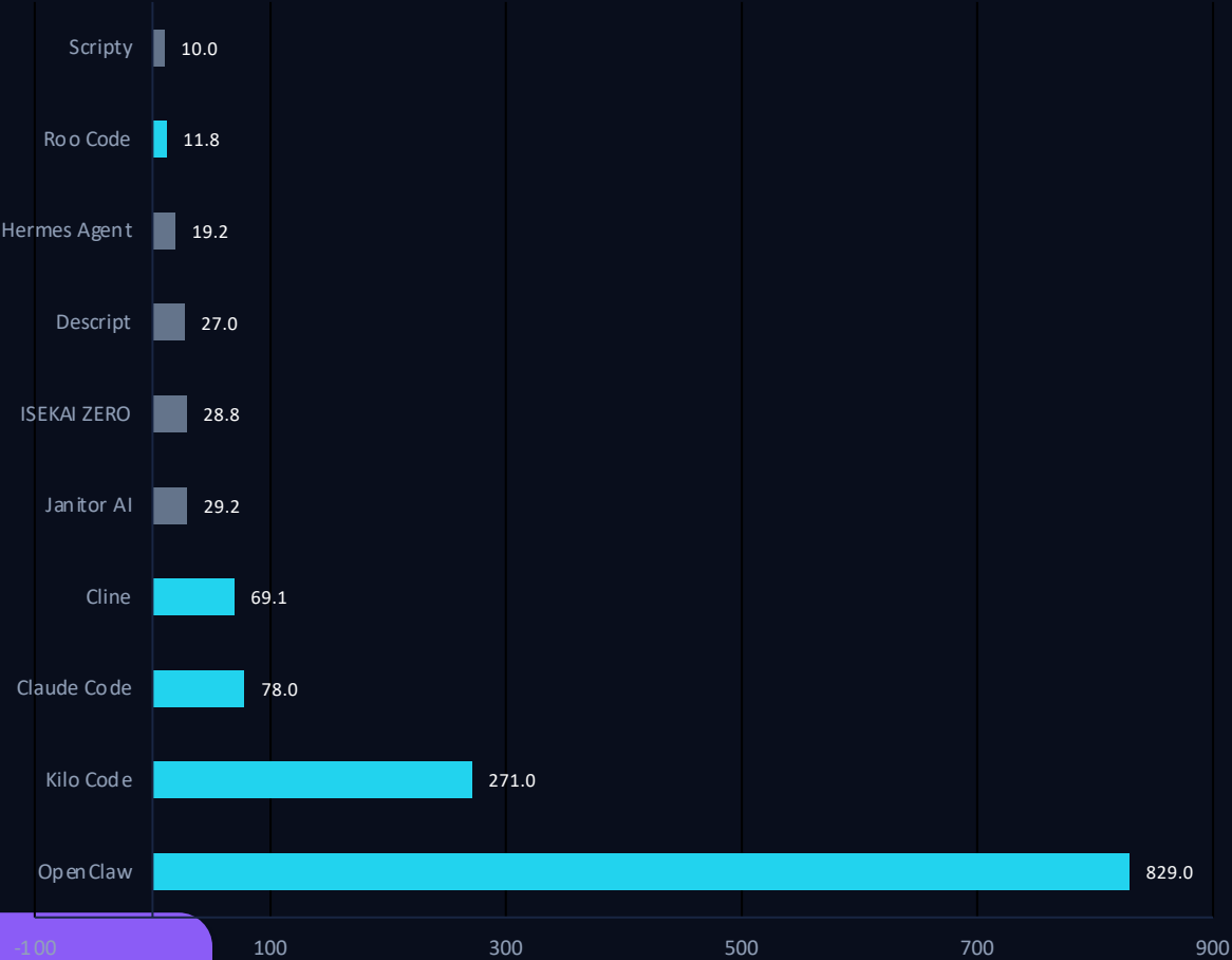
Daily tokens (B)
