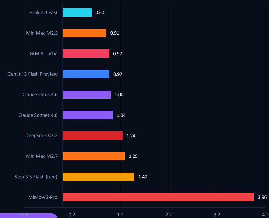
Weekly token usage (T)
