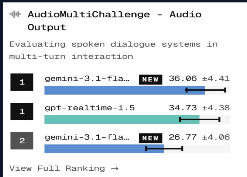
AudioMultiChallenge Output (Figure 1)
